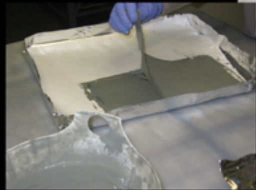
Wet lay-up
